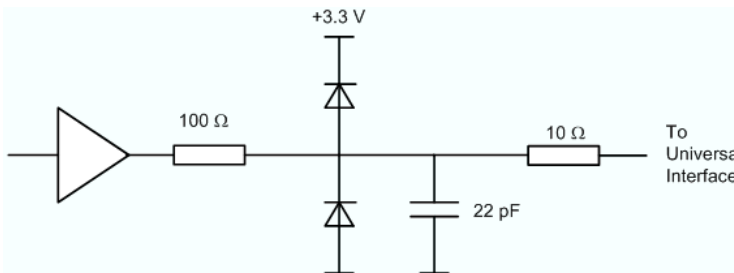
Circuit diagram of the output path
