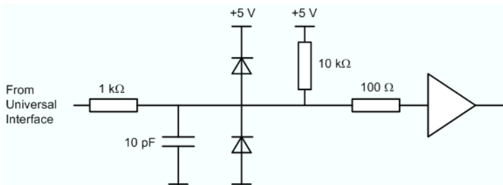
Circuit diagram of the input path
